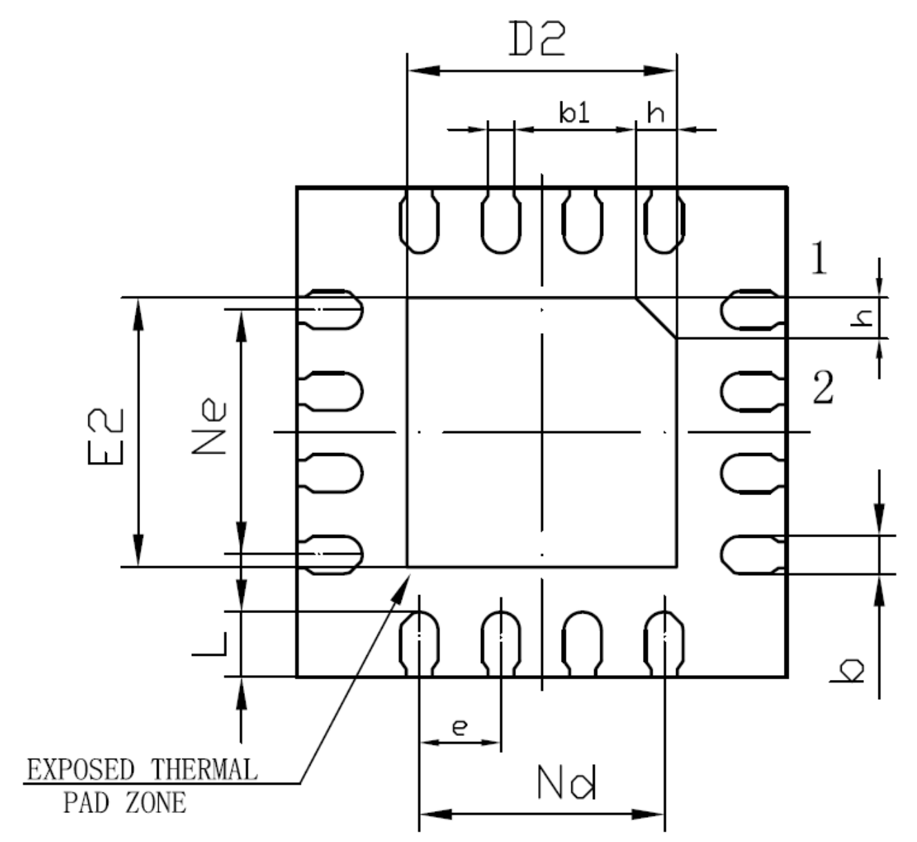
BOTTOM VIEW
